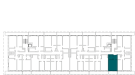
FLOOR PLAN
